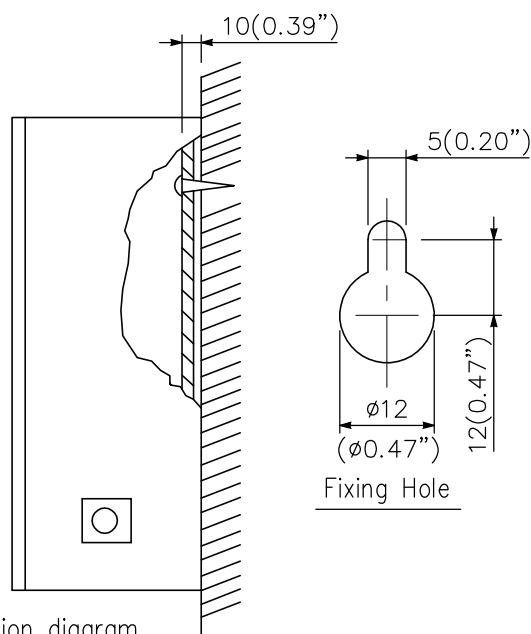
Installation diagram
