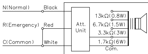
2-wire system
