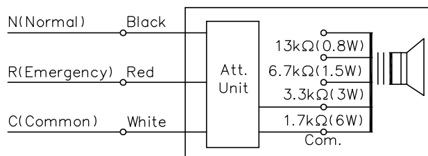
3-wire system
