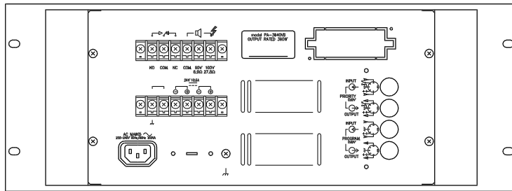
Rear View
